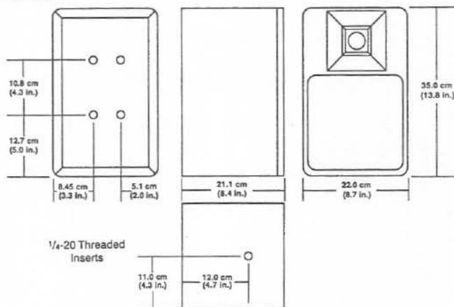
FIGURE 8 — Dimensions
