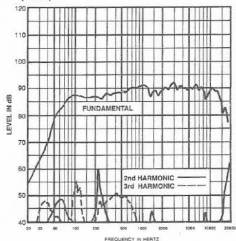
FIGURE 5 — Harmonic Distortion, 0.01 Rated Power Input (1 watt)
