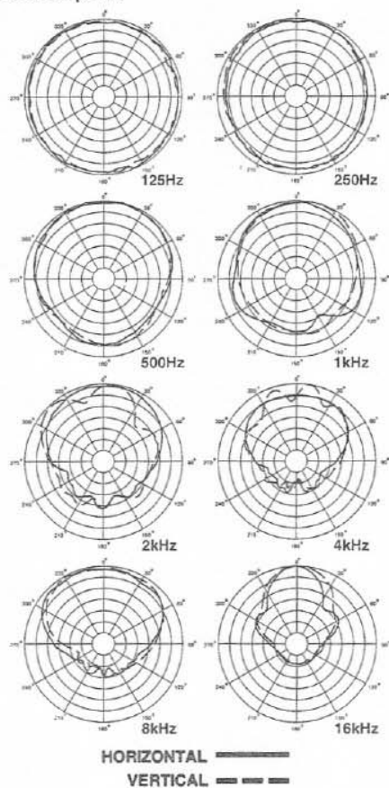
FIGURE 2 — Polar Response
